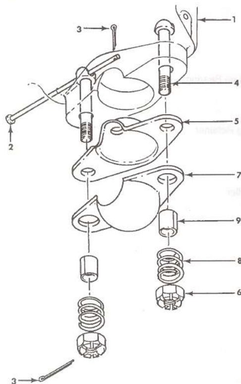
MODEL A FORD FRONT RADIUS ROD BALL SOCKET ASSEMBLY 1928-1931
