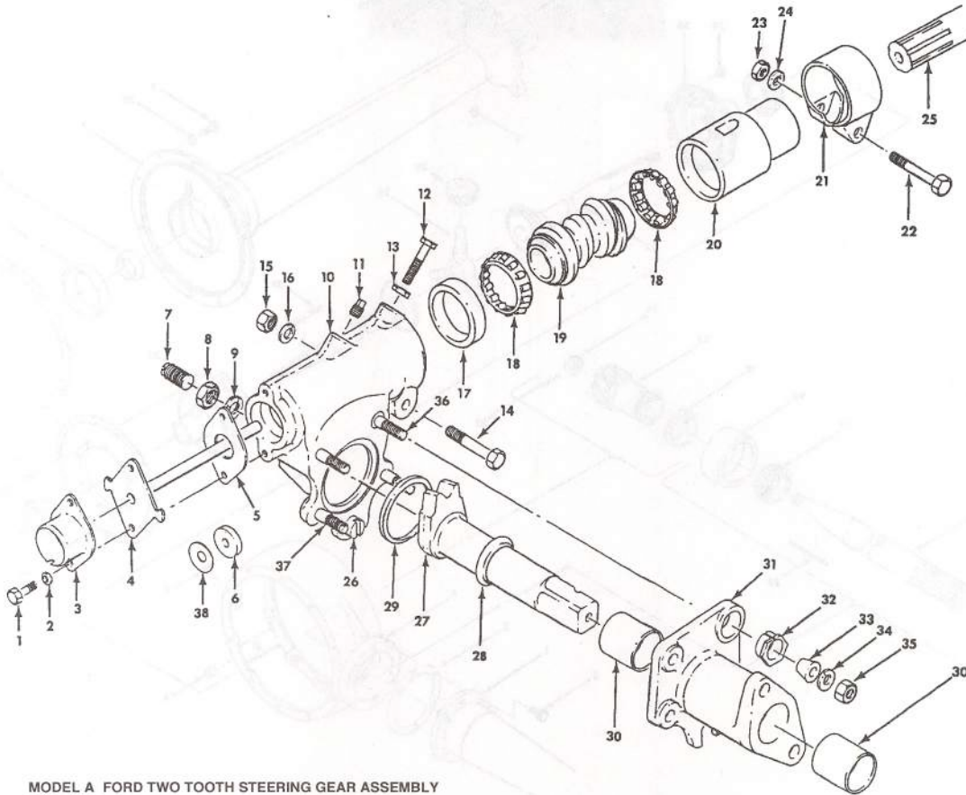
MODEL A FORD TWO TOOTH STEERING GEAR ASSEMBLY 1929-1931
