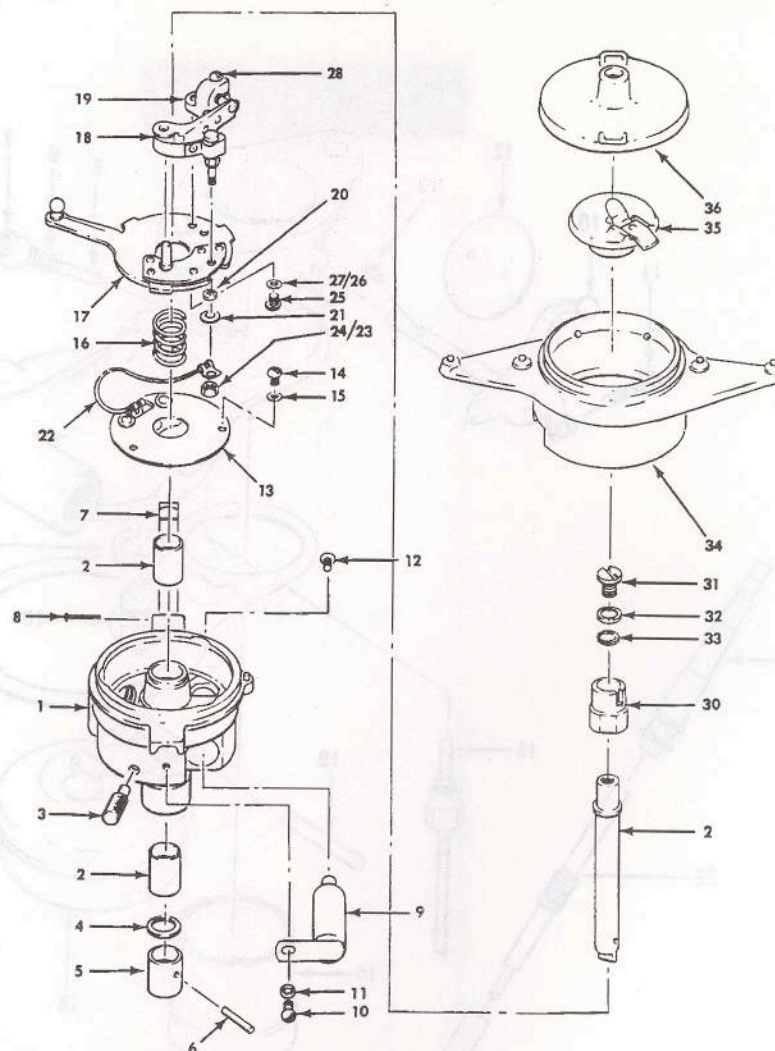
MODEL A FORD DISTRIBUTOR ASSEMBLY 1928-1931
