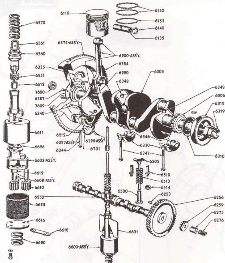
4-Cylinder Motor
