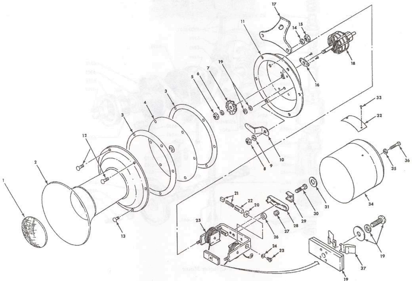
MODEL A FORD HORN ASSEMBLY - SPARTON 1928-1931 P/N A-3305
